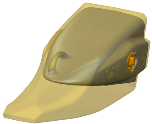
X220 Heavy Penetration Tip 60% Available Wear Material
